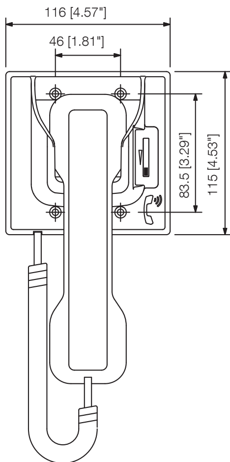
Front View
