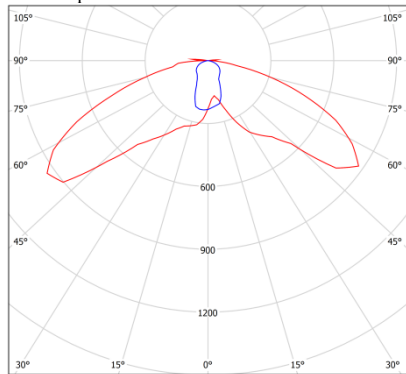
L1 cd/klm CO - C180 C90 - C270 η = 100%
