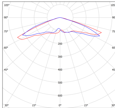
L2 cd/klm CO - C180 C90 - C270 η = 100%
